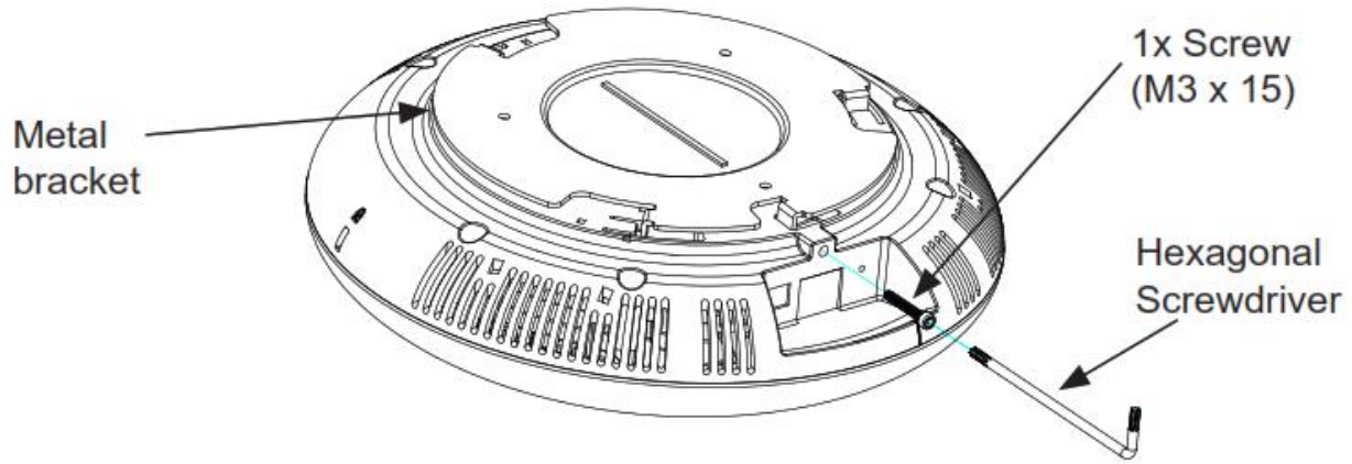
Figure 11: Anti-theft Installation
