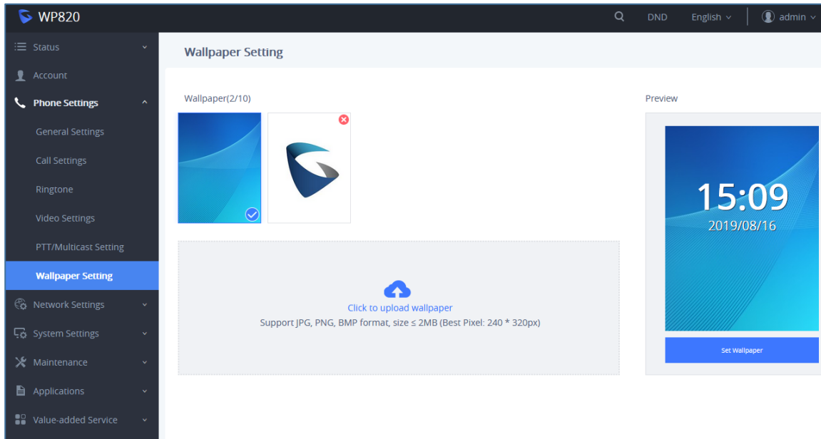
Figure 45: Deleting Wallpaper
