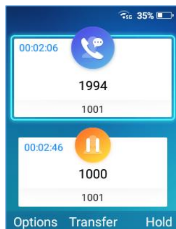
Figure 58: Split Calls
