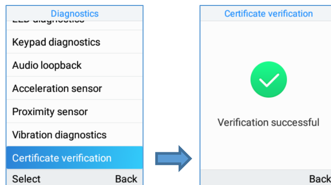
Figure 104: Certificate Verification
