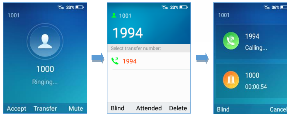
Figure 57: Attended transfer
