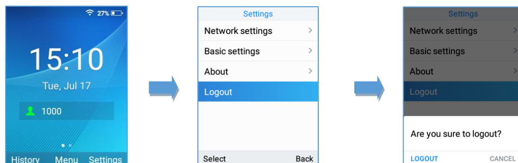
Figure 34: Guest Logout
