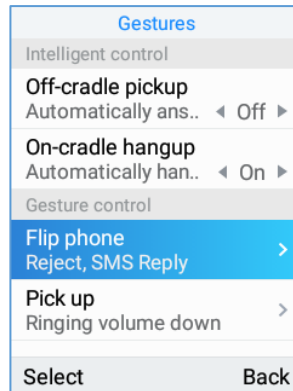
Figure 90: Flip Phone
