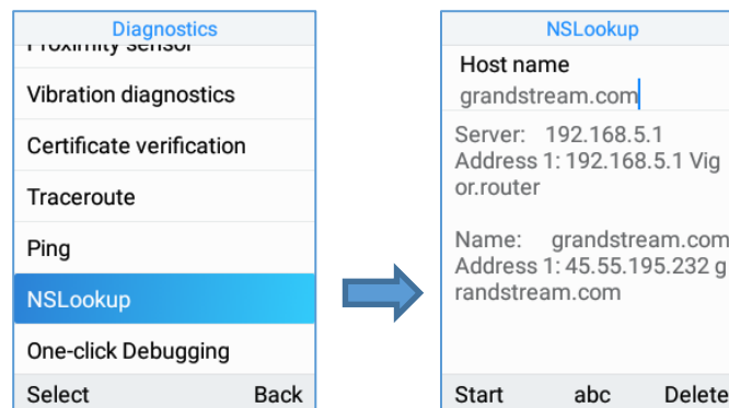
Figure 107: Nslookup
