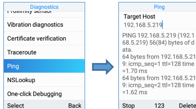
Figure 106: Ping
