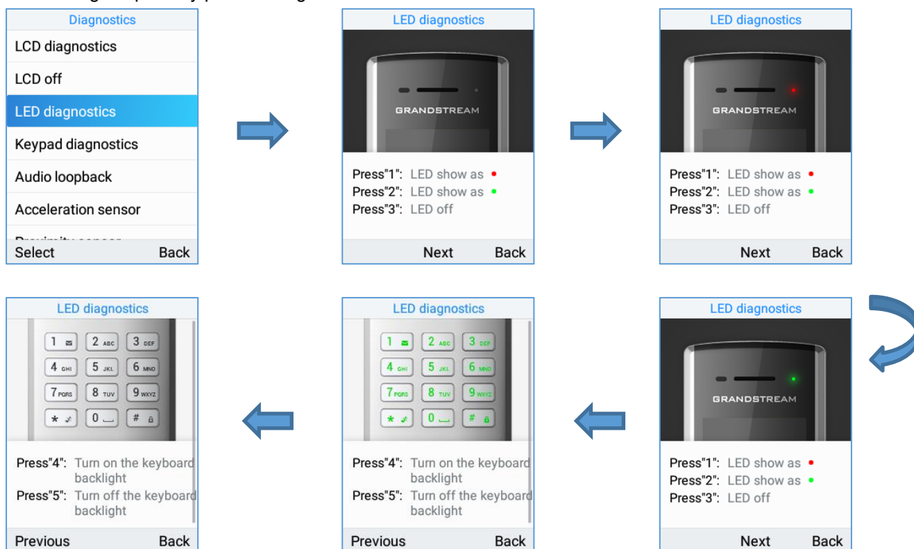
Figure 98: LED Diagnostics
