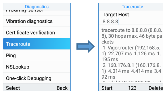
Figure 105: Traceroute
