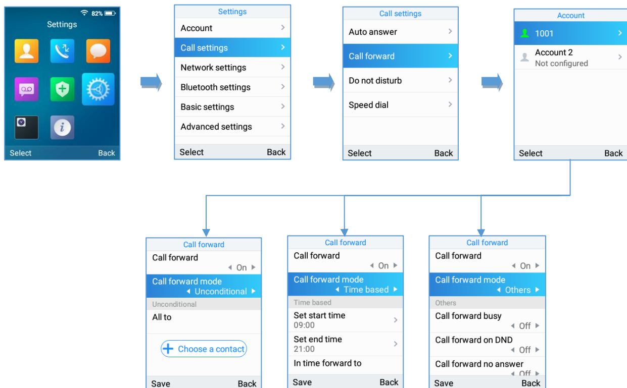
Figure 54: Call Forwarding
