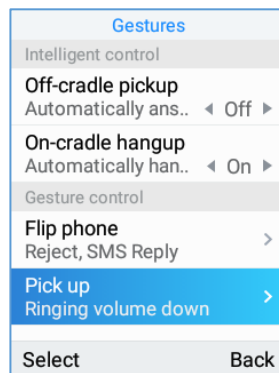
Figure 92: Pick up
