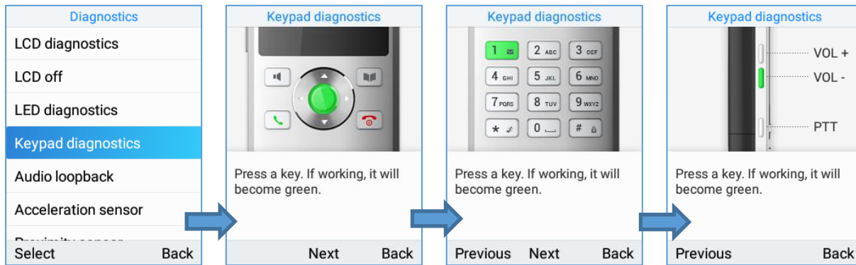
Figure 99: keypad Diagnostics
