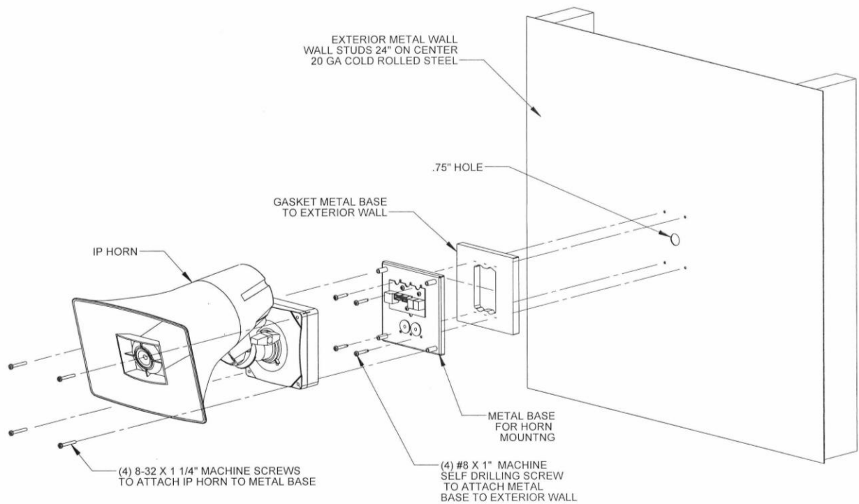
Figure 4. Exterior Mounting
