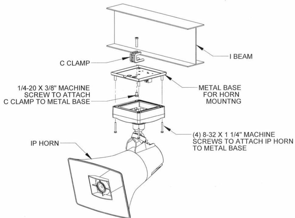
Figure 5. Interior I-Beam Mounting
