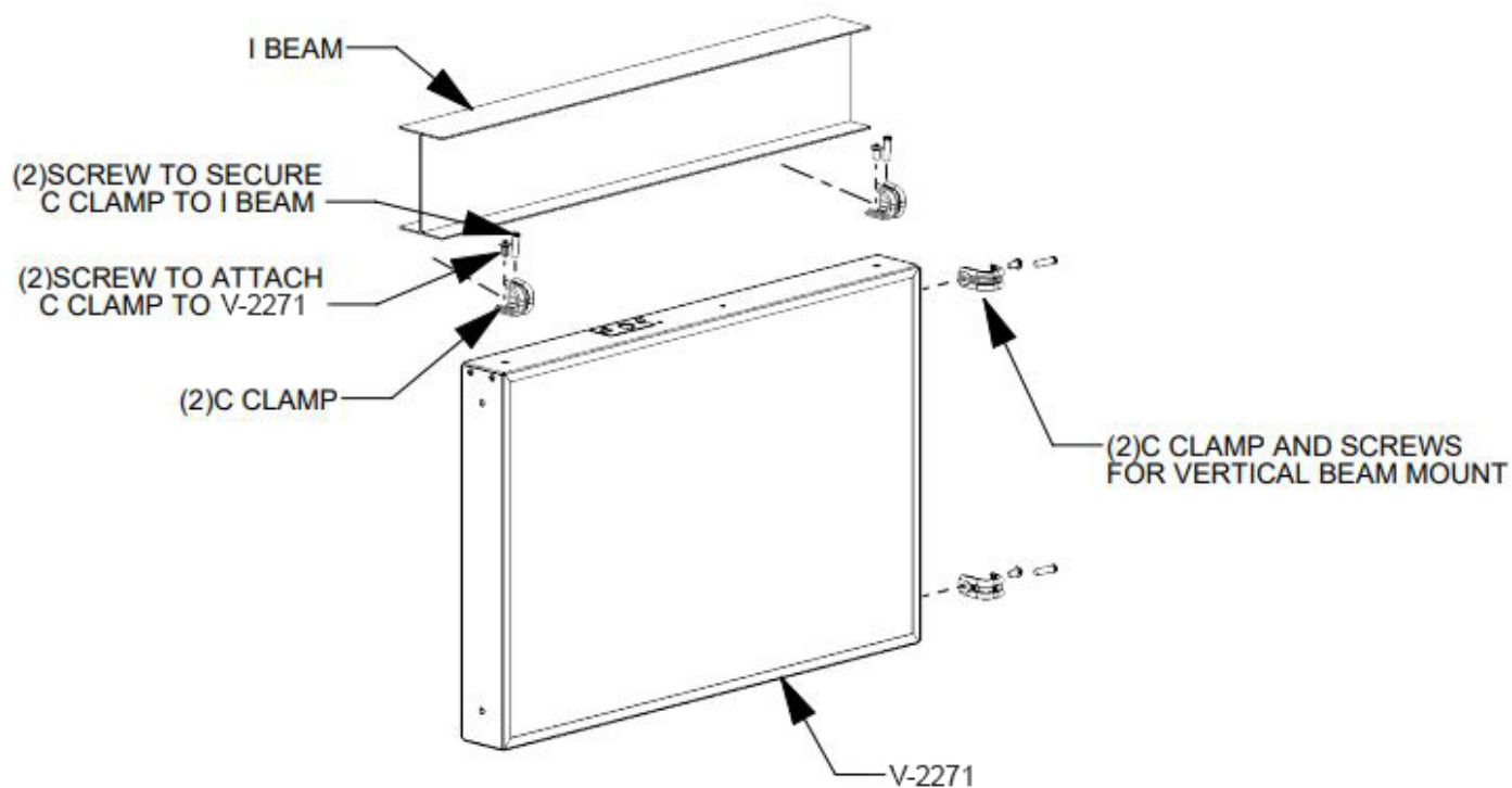
Figure 2: Beam Mounting
