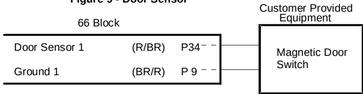
Figure 9 - Door Sensor
