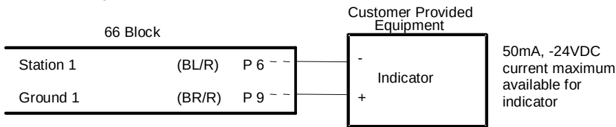
Figure 8 - Handsfree Indicator
