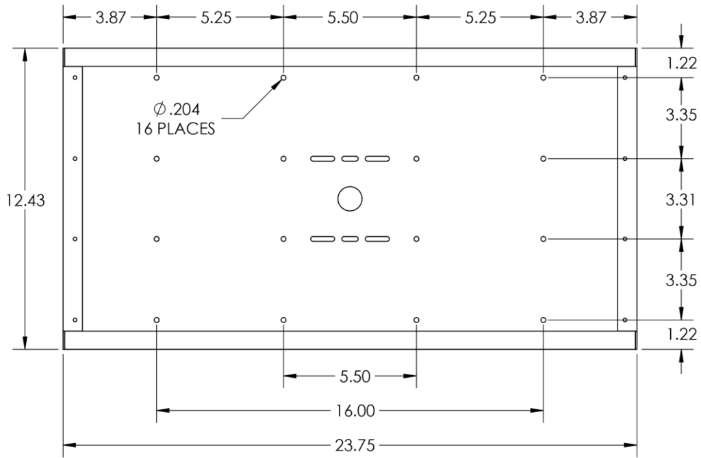
Figure 1. Backbox Mounting Hole Dimensions
