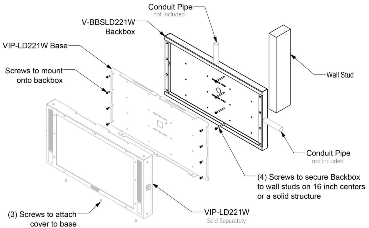
Figure 2. Backbox Assembly
