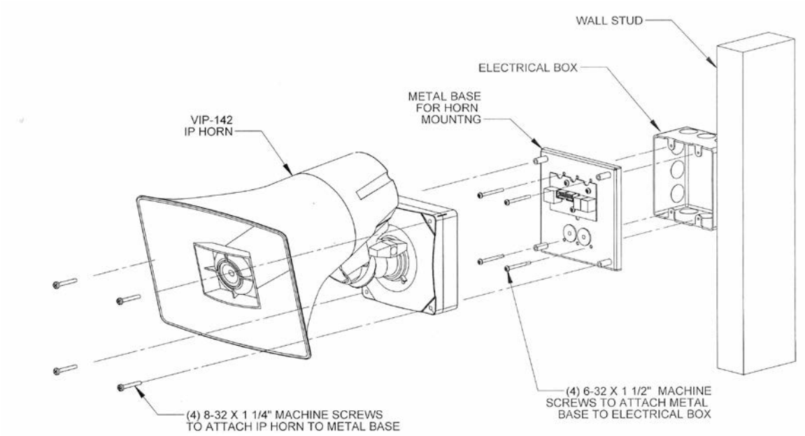
Figure 3. Interior Mounting
