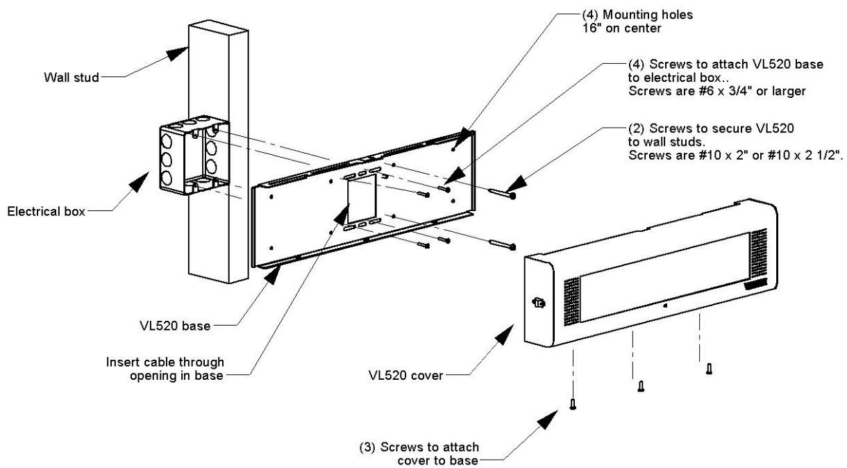
Figure 2. Mounting Diagram
