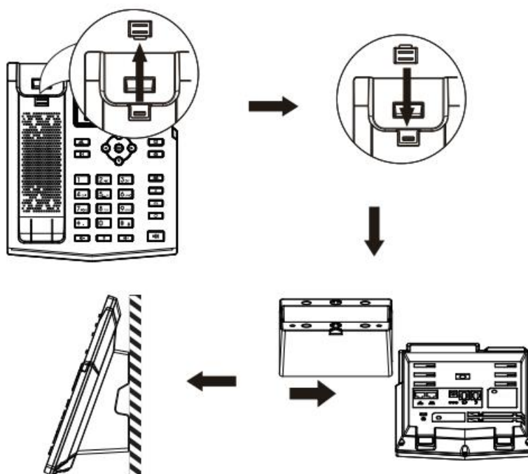
Picture 2 - Wall-mounted installation
